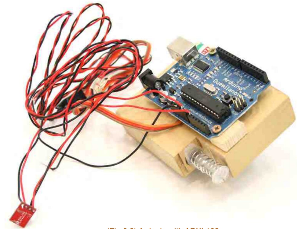
(Fig 6.2) Arduino with ADXL193
